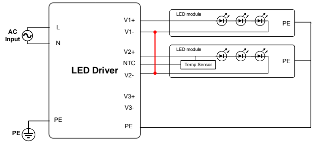
Misconnection of all 2 output negative terminals together.
