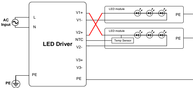
Cross misconnections between all 2 channels.
