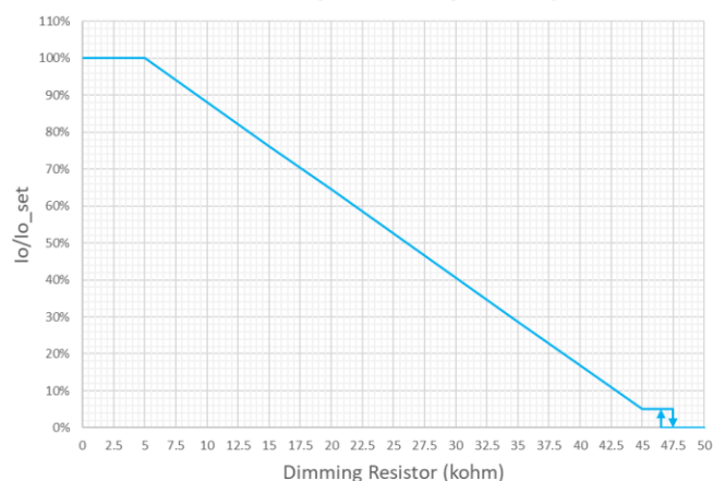
Resistor Dimming Curve (Negative Logic)
