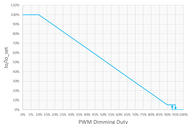
PWM Dimming Curve(Negative Logic)
