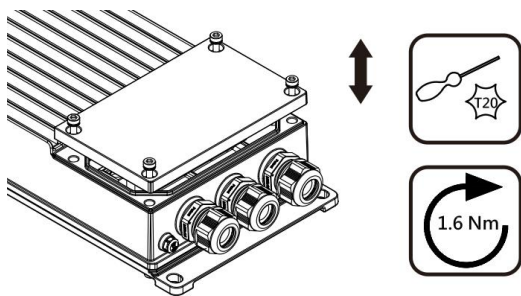
0~10V/PWM Model Connection
