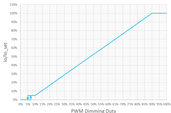
PWM Dimming Curve(Positive Logic)
