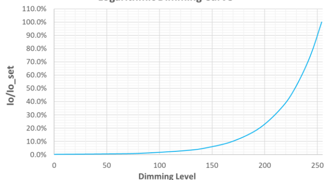
Logarithmic Dimming Curve
