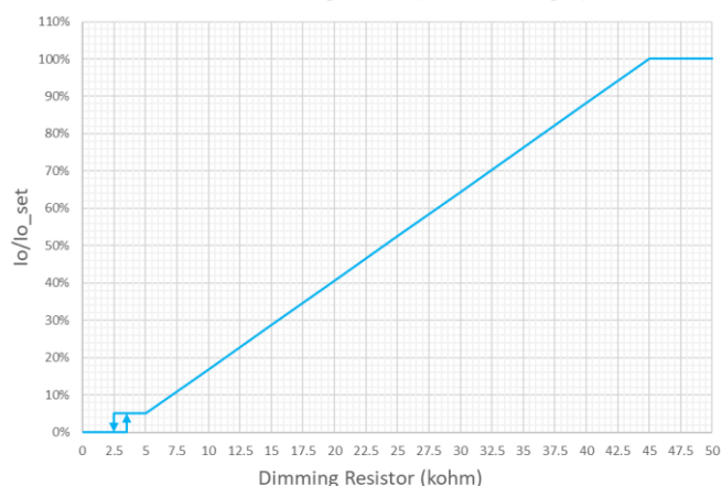
Resistor Dimming Curve (Positive Logic)
