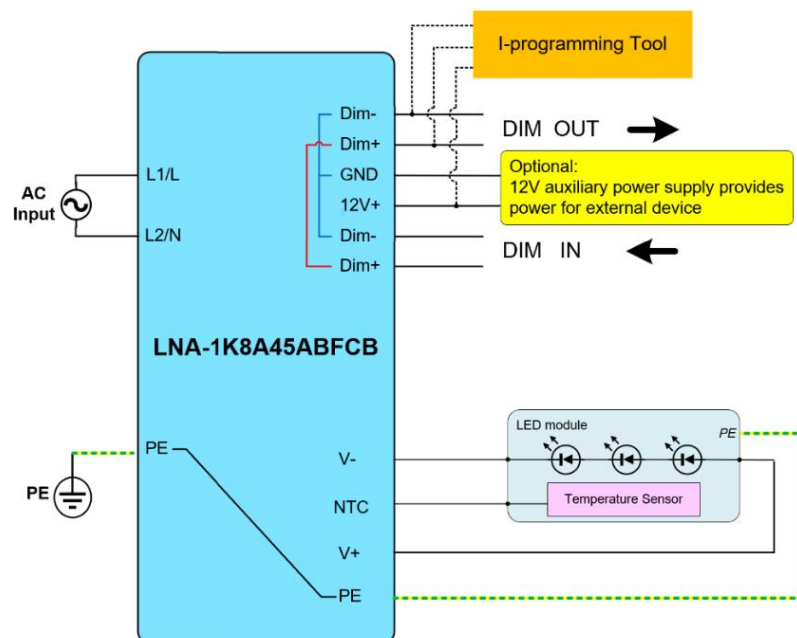
(a) 0-10V/PWM/Resistor Mode
