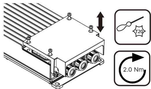
0~10V/PWM Model Connection
