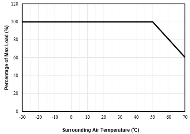
Fig. 1.3 De-rating for Mounting Orientation A to F > 50°C de-rate power by 2% / °C
