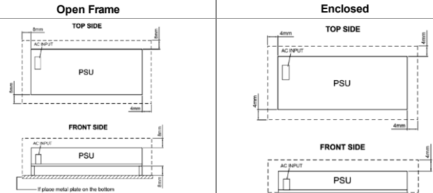
Fig. 2: Assembly Reference
