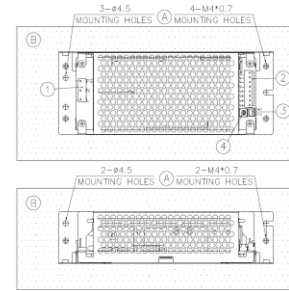
PJ-□□V100WDRA: Open Frame
