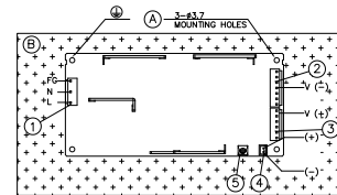
Fig. 1: Device Descriptions
