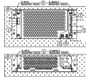
PJ-□□V150WERA: Enclosed (with cover and chassis)
